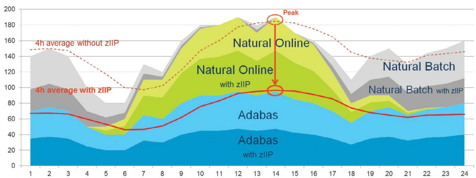
Figure 3: Reduce Peak Workload with zIIP Offloading
